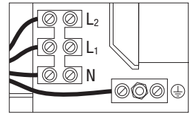
Electrak 31, 3P+E
