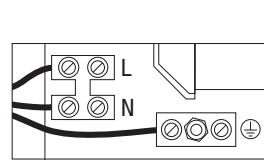
Electrak 30, 2P+E
