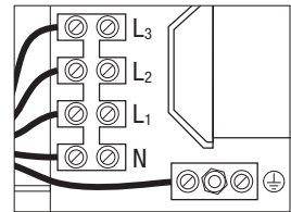
Electrak 33, 4P+E
