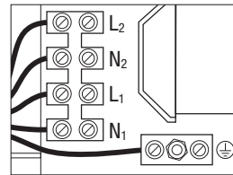
Electrak 32, 4P+E
